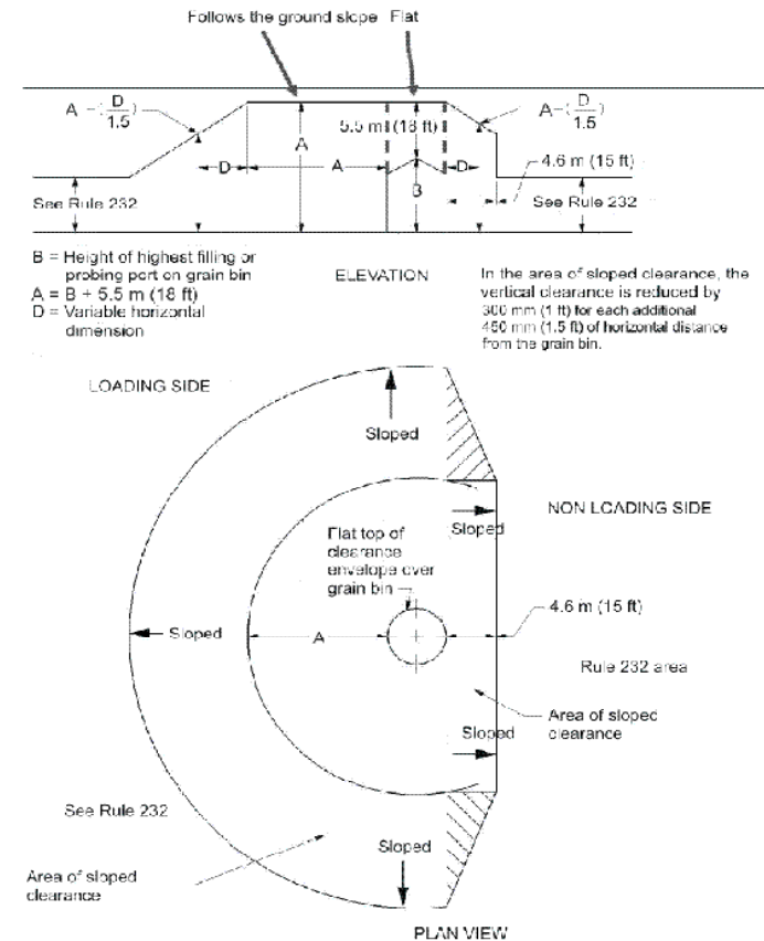
Figs. 234-4(b) Clearance Envelope for Grain Bins Filled by Portable Augers, Conveyors, or Elevators
